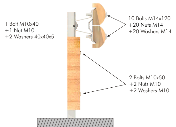
Detail of joint between barriers
